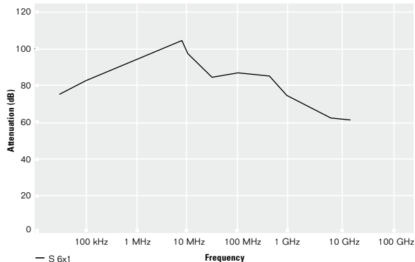
SHIELDING EFFECTIVENESS
