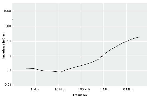
TRANSFER IMPEDANCE
