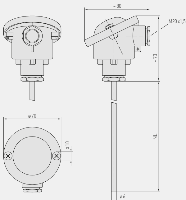
Dimensional drawing
